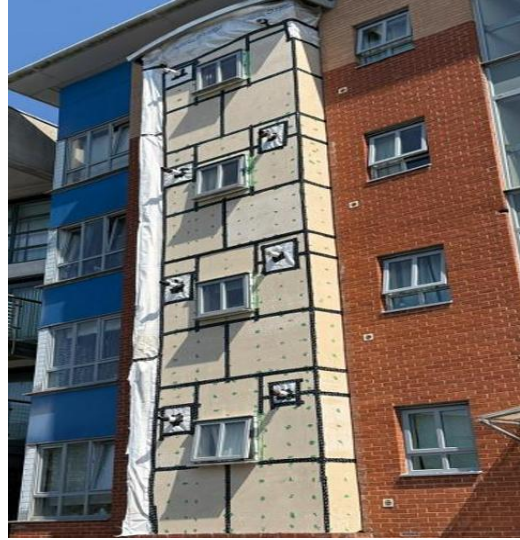
A photo showing Panels stripped and CP Board installed
